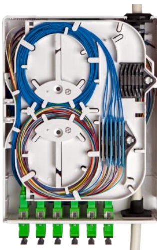
Easy box 24S/12C (24 splices; 6x SC duplex)
